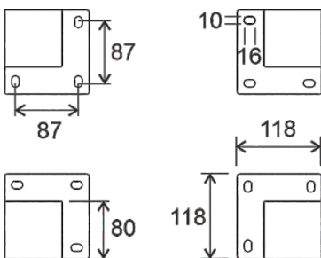
Floor installation brackets
