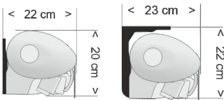
Wall / ceiling installtion size
