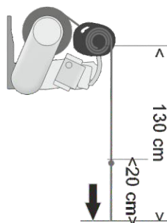
Vario-volant Rollable valance (manual/electric)
