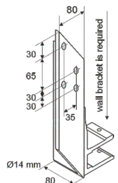
Rafter adapter
