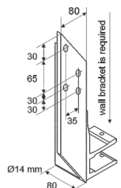
Rafter adapter
