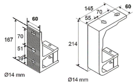
Wall / ceiling brackets
