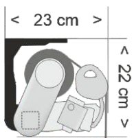
Wall / ceiling installation size
