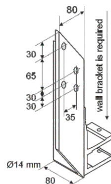
Rafter adapter
