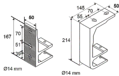
Wall / ceiling brackets
