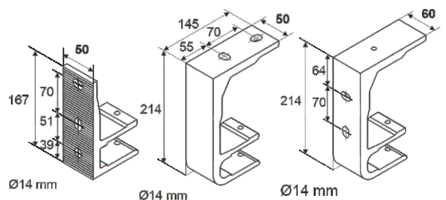
Wall / ceiling / roofing brackets
