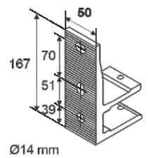
Wall brackets
